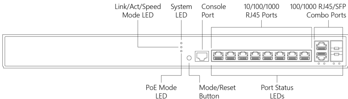
Figure 1: Front panel of the switch
